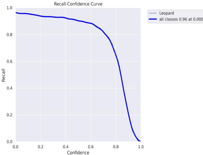
Figure 3- Recall-Confidence Curve
