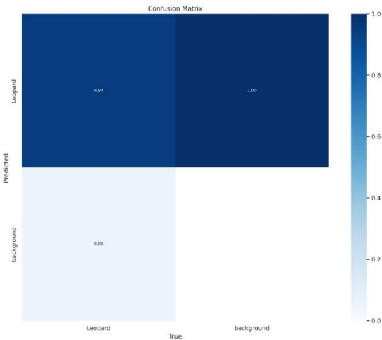
Figure 4- Confusion matrix
