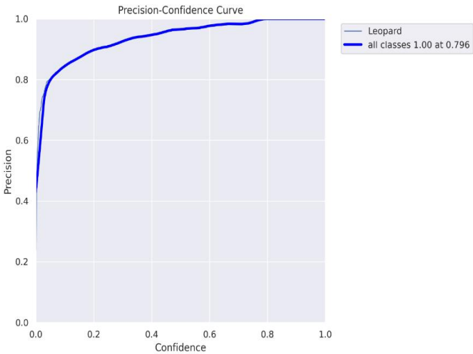
Figure 2- Precision-Confidence Curve
