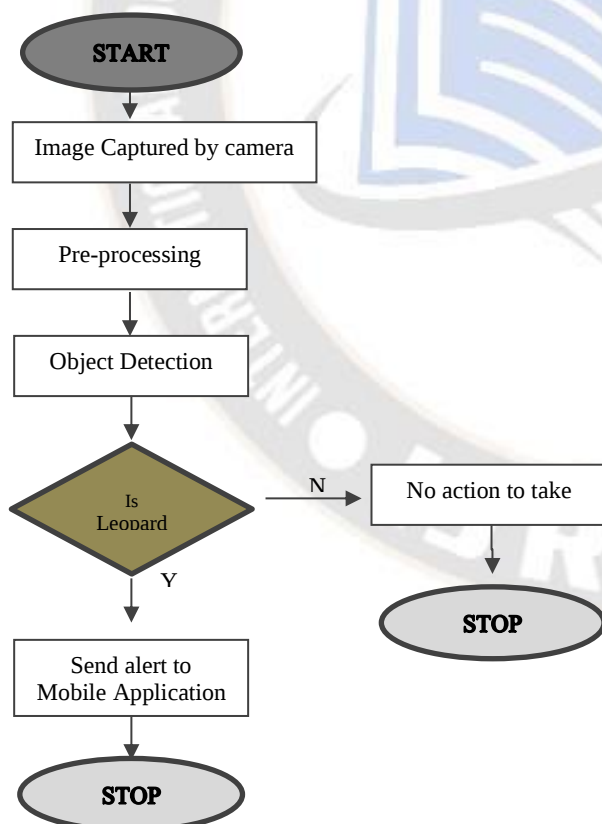
Figure 1. Proposed Architecture
